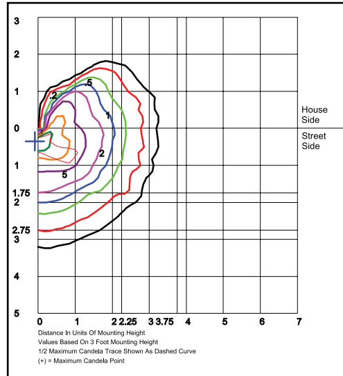
B5HQB1X16U5K 180° Shield - Clear Glass Lens Grid in feet, Mounting Height = 3 ft.
