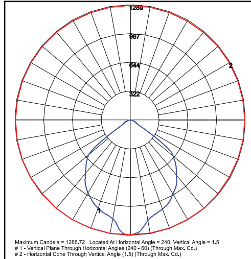
WCTRSBC31X20U41K 100° Reflector
