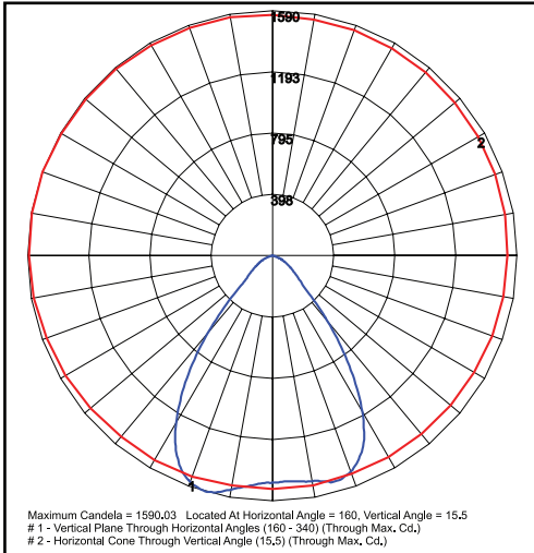
WCTRSAC31X20U41K 70° Reflector
