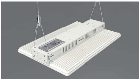
Mounting With Aircraft Cable (Standard)
