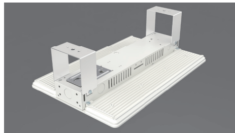
Surface Mounting SM-LH07-130W (FOR 130W) SM-LH07-300W (FOR 160W, 205W, 250W, 300W)
